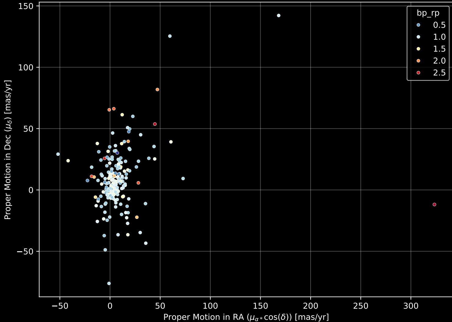
APOGEE DR17 Field: [265-37-O_TESS] Proper Motion Diagram (n= 205)
