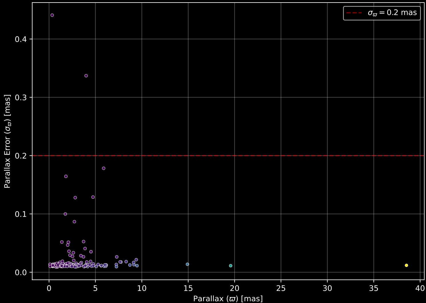
APOGEE DR17 Field: [265-37-O_TESS] Parallax Quality (n= 205)
