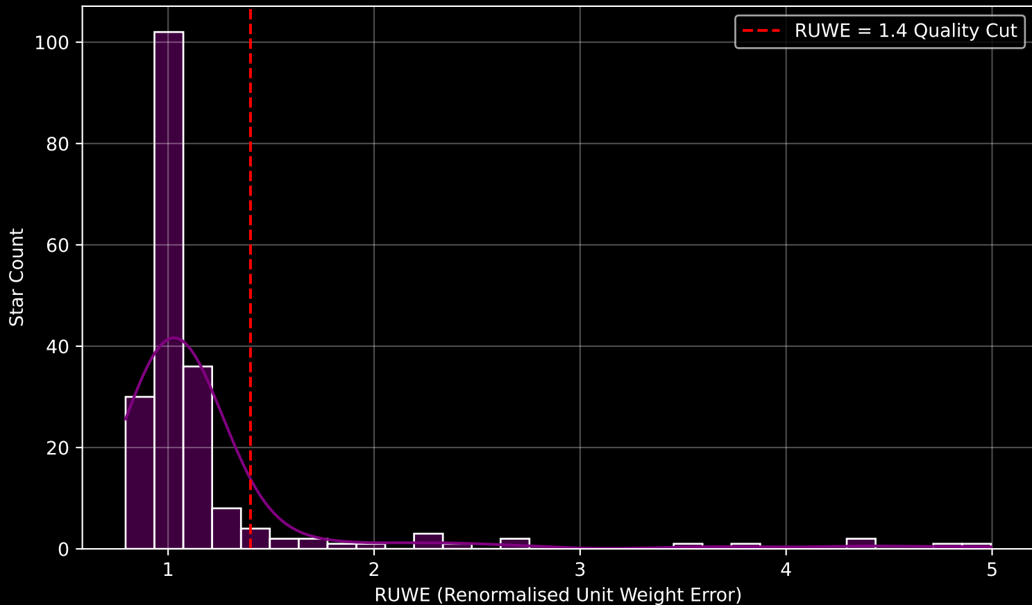
GAPOGEE DR17 Field [265-37-O_TESS] RUWE Distribution (n= 198)
