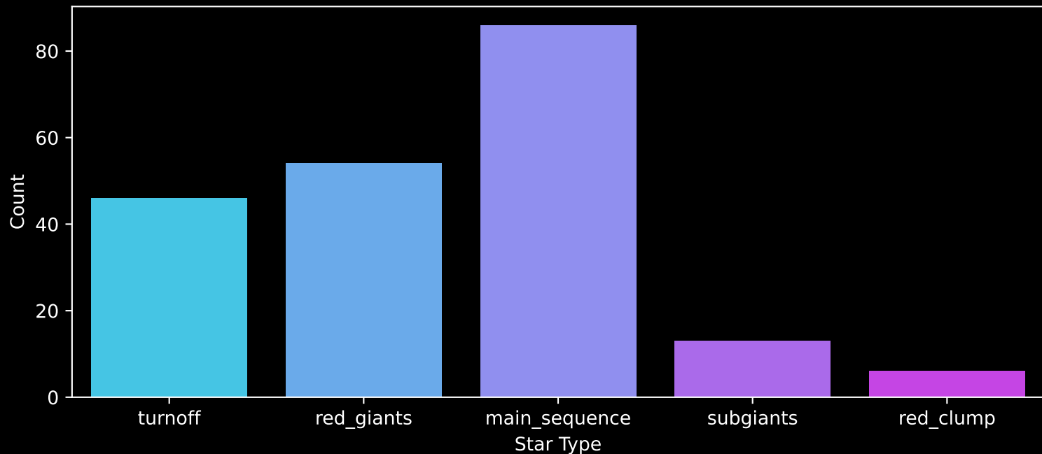
APOGEE DR17 Field: [265-37-O_TESS] Count plot of Star Type
