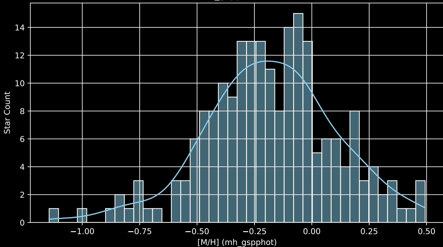
APOGEE DR17 Field: [265-37-O_TESS [M/H] (mh_gspphot) (n= 204)
